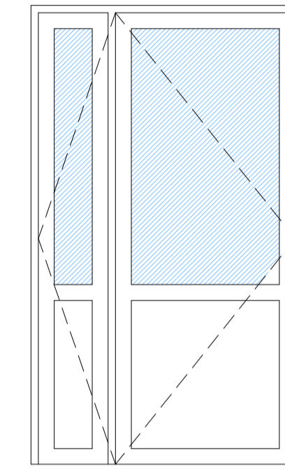
Proposed Hall Entrance (3) 1:25
