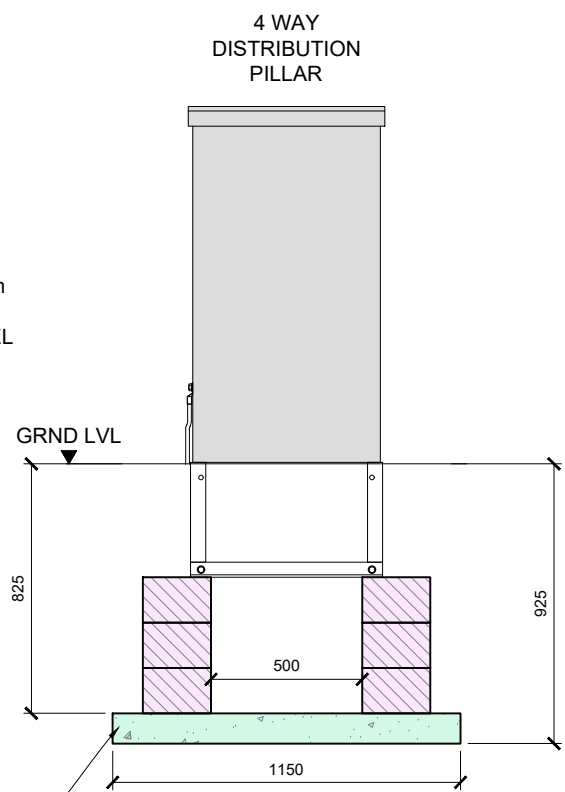
REAR VIEW
