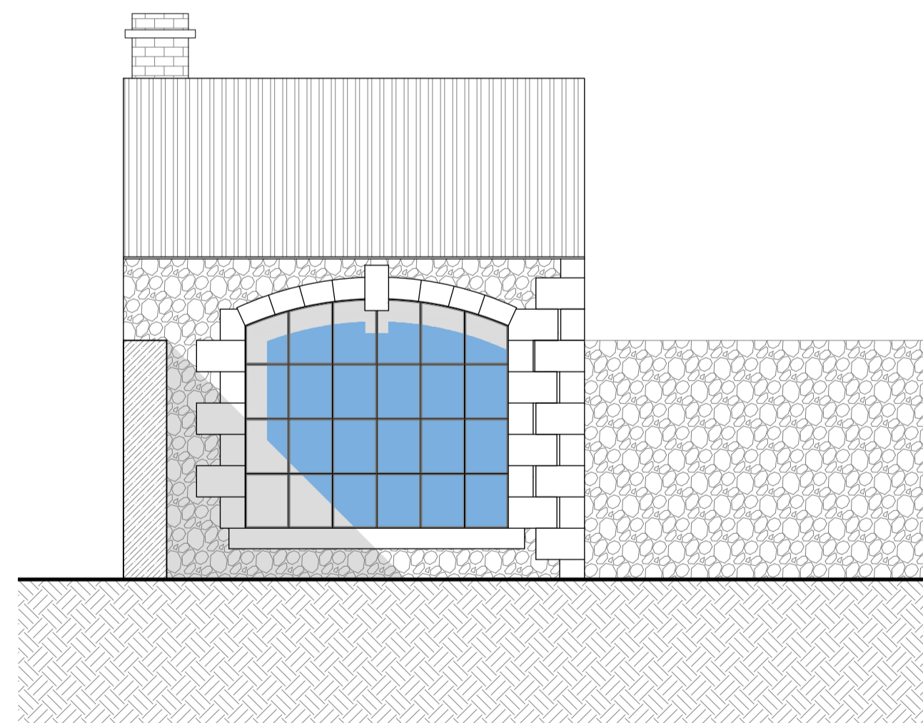
Existing Outbuilding West Elevation SCALE 1:50
