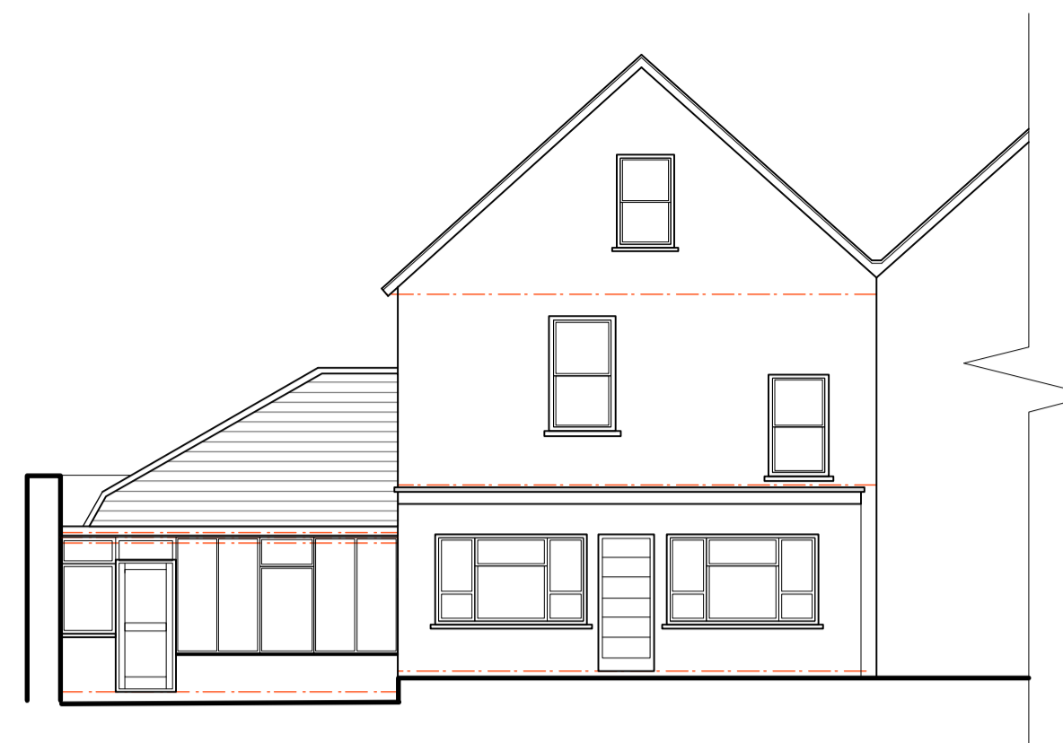
NORTH ELEVATION
