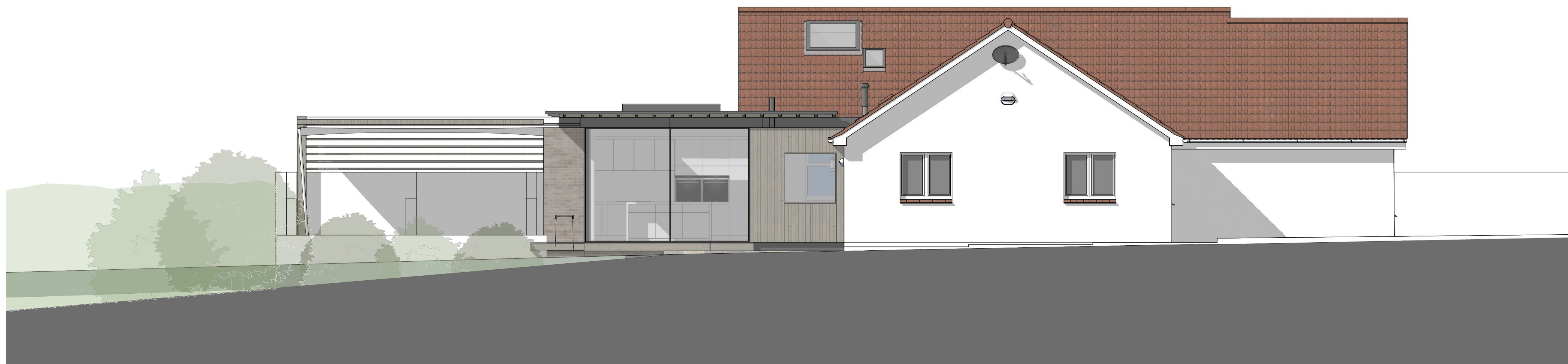
South Elevation
