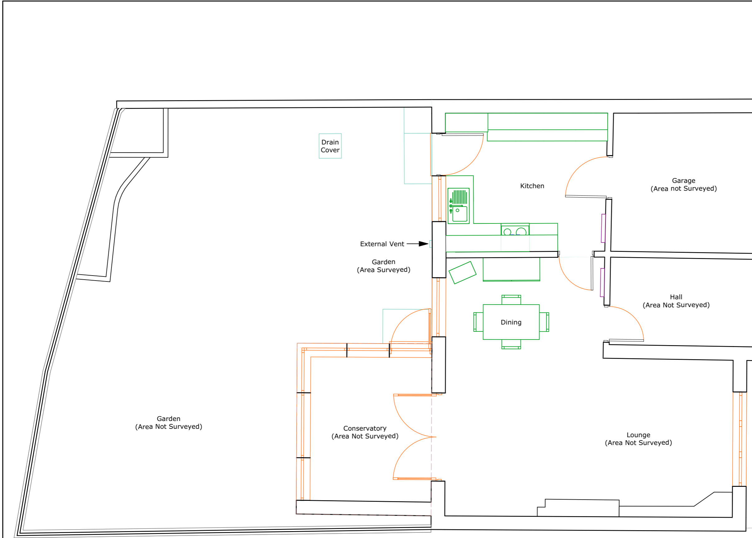
Ground Floor Survey Plan
