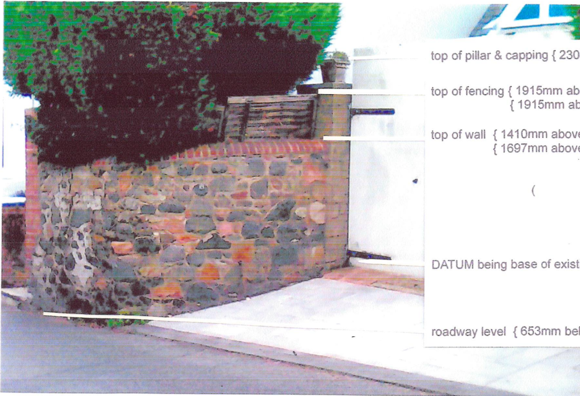
FIGURE 3A Photograph of Existing Damaged Wall Section annotated to show wall and fencing heights
