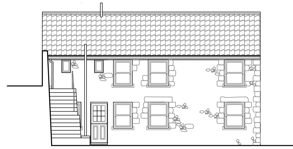
South Elevation 1:100
