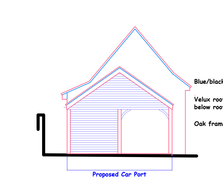
WEST ELEVATION 1 : 100
