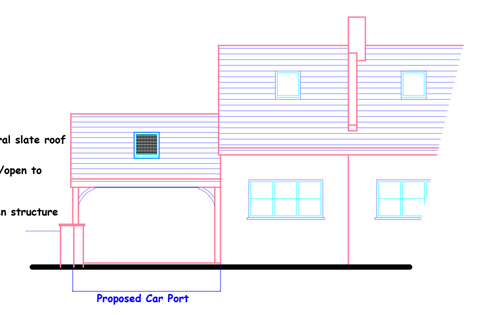
SOUTH ELEVATION 1 : 100
