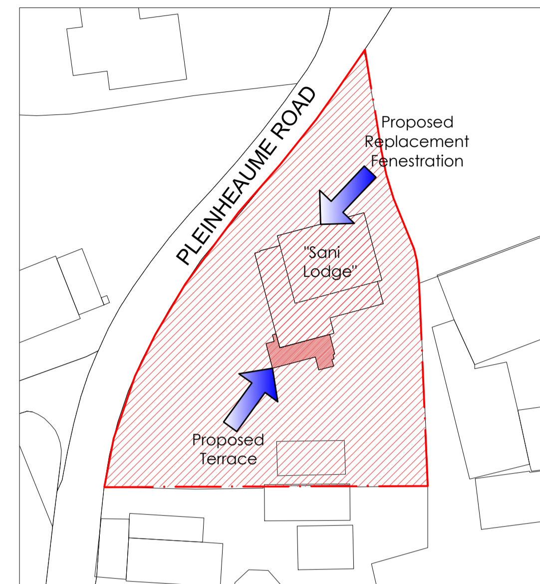
Block Plan 1:500
