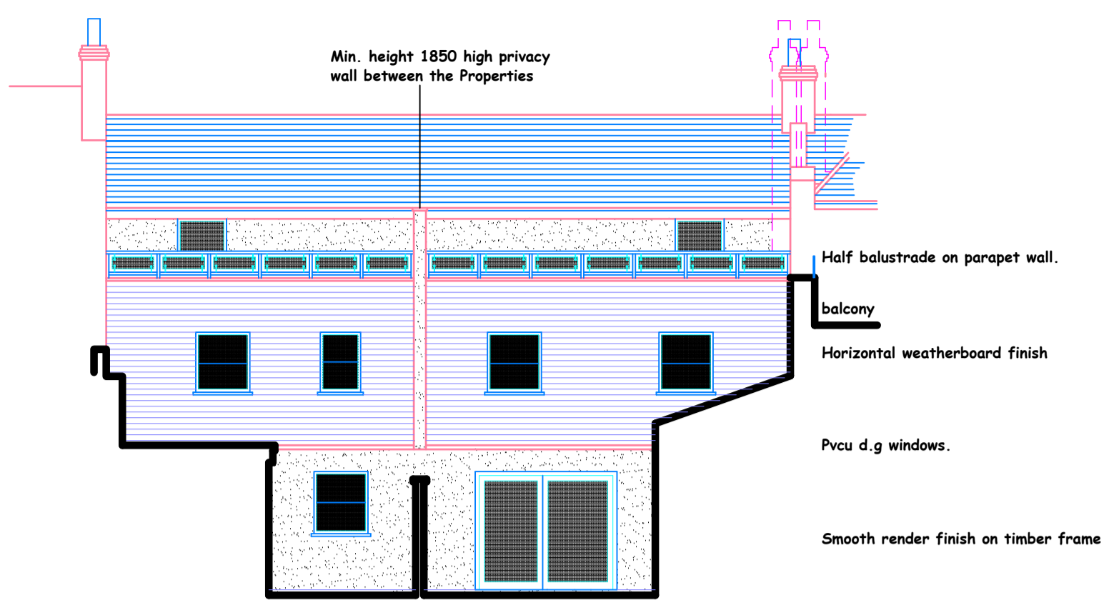
EAST ELEVATION
