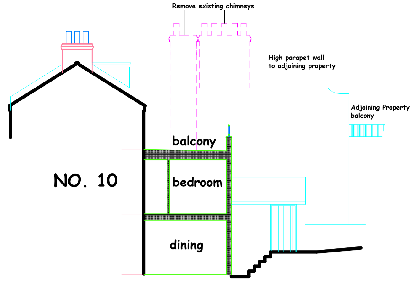
NORTH SECTIONAL ELEVATION BB
