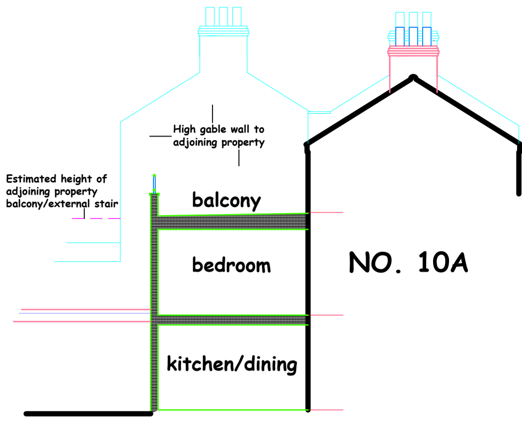
SOUTH SECTIONAL ELEVATION AA
