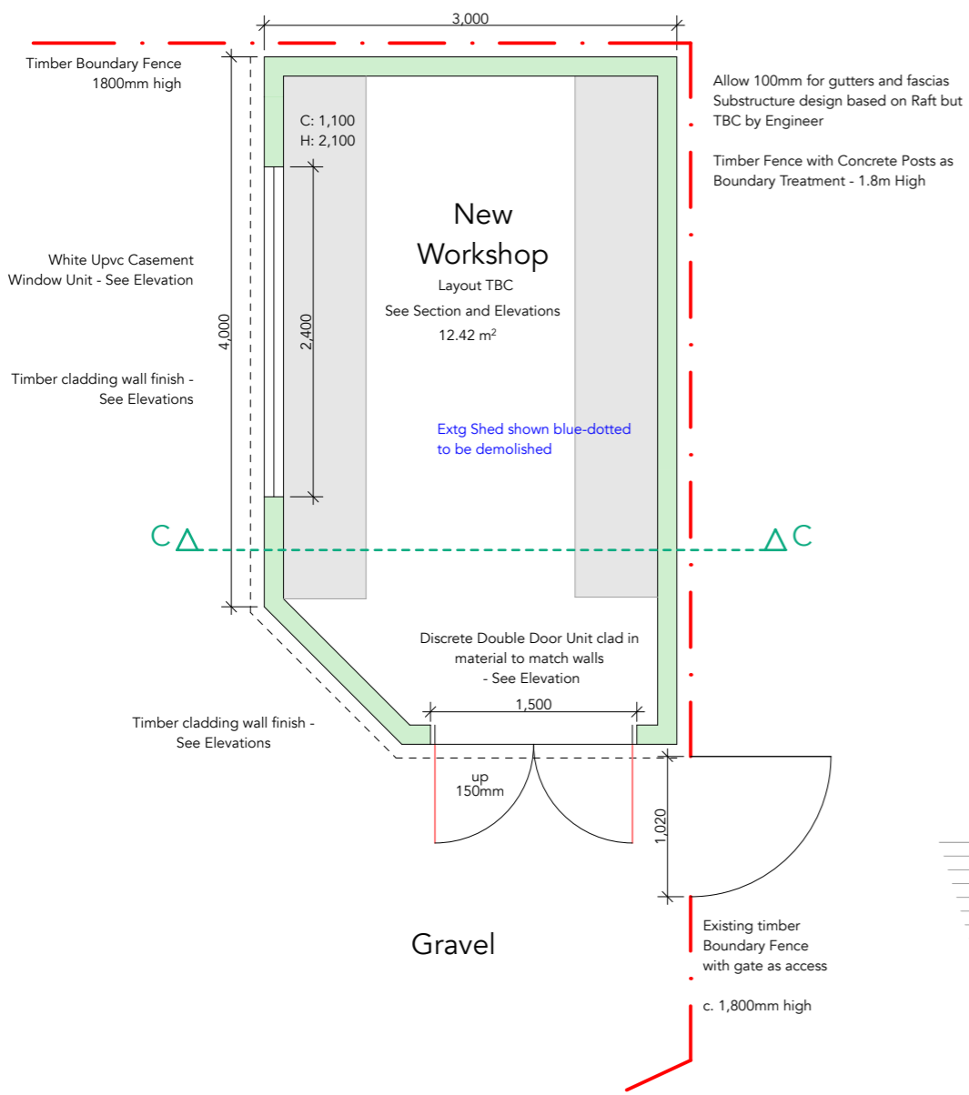
Proposed Part Site Plan Scale:- 1:50
