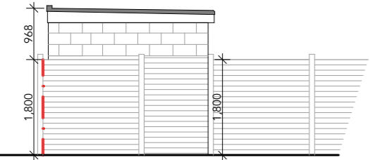
Proposed: S-W Elevation
