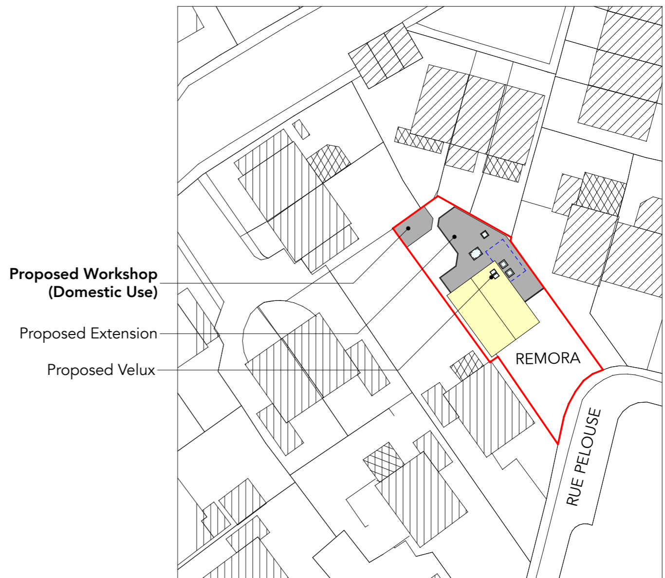
Block Plan
