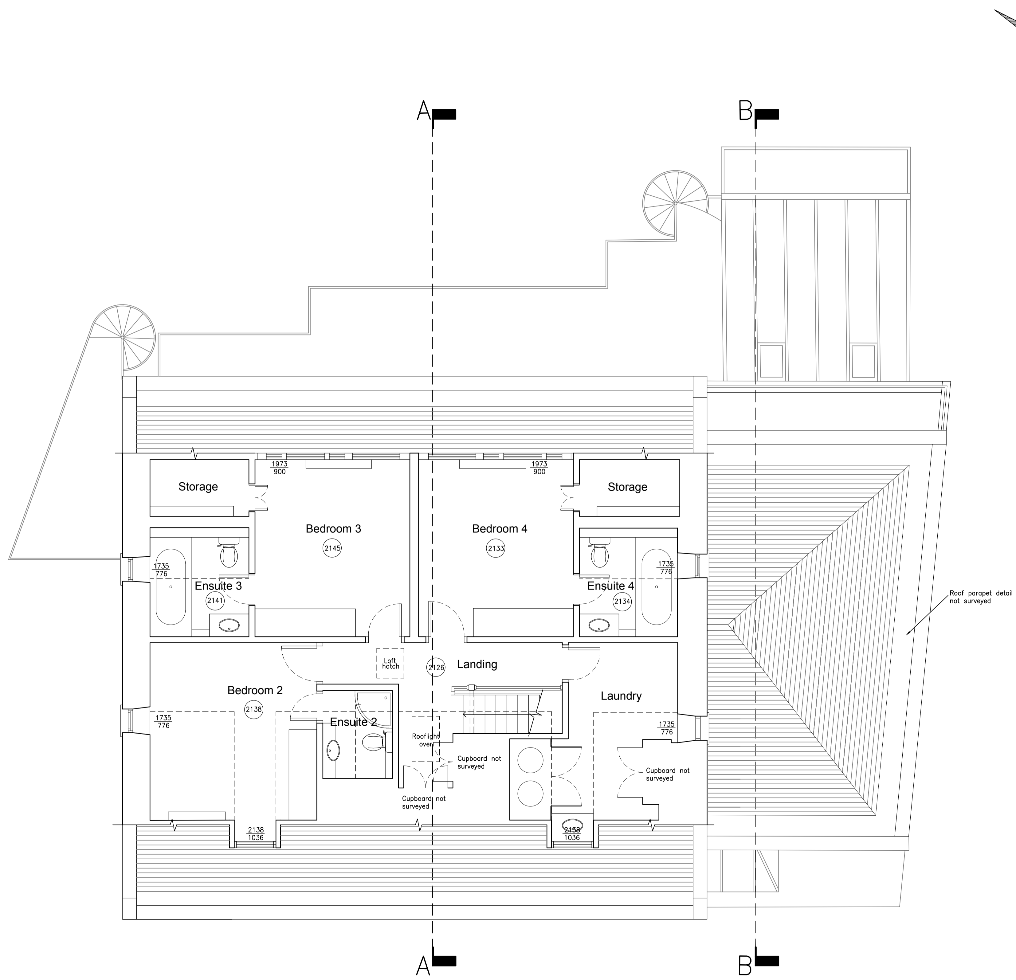
Second Floor Plan Scale 1:50
