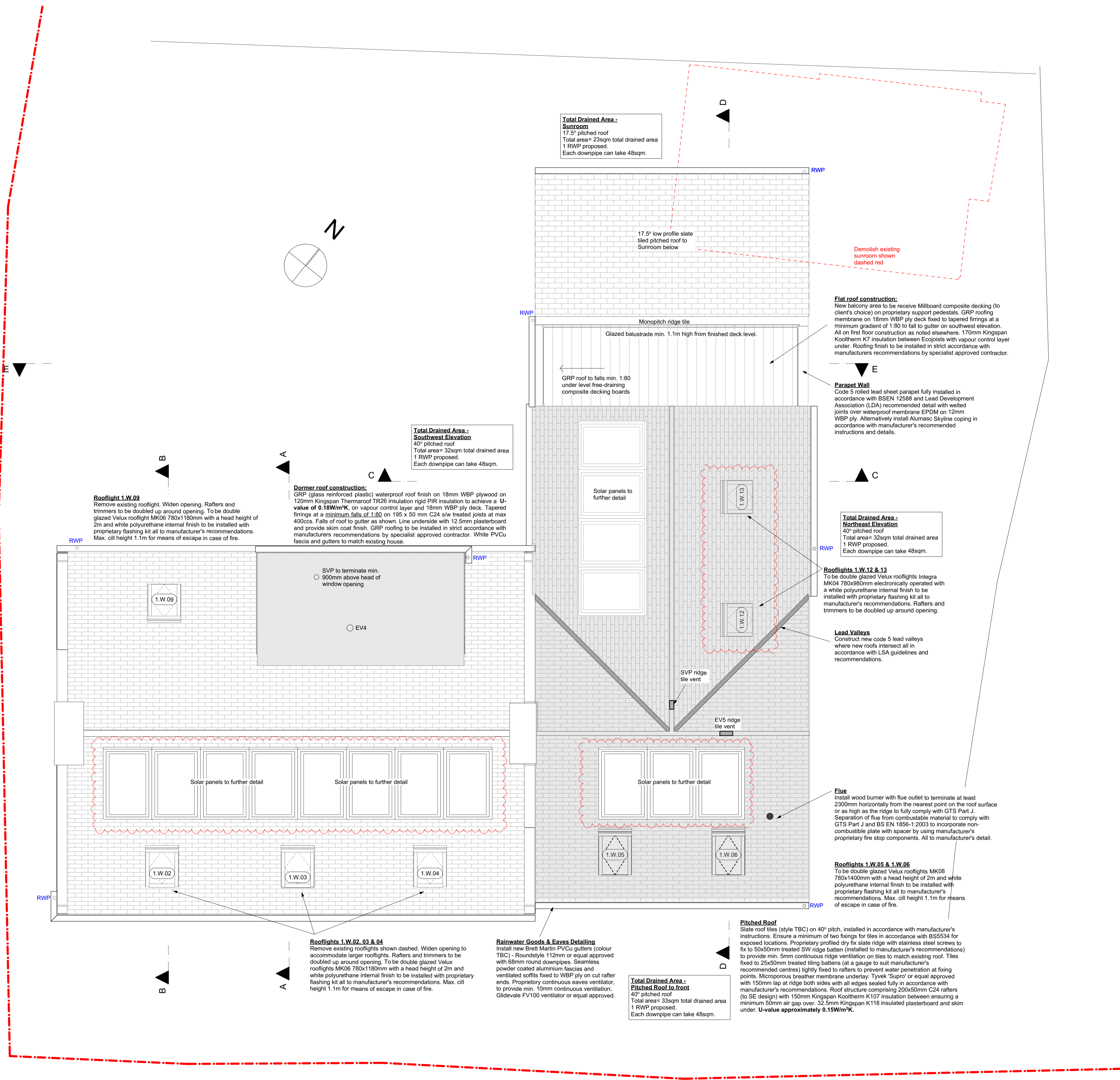
Proposed Roof Plan
