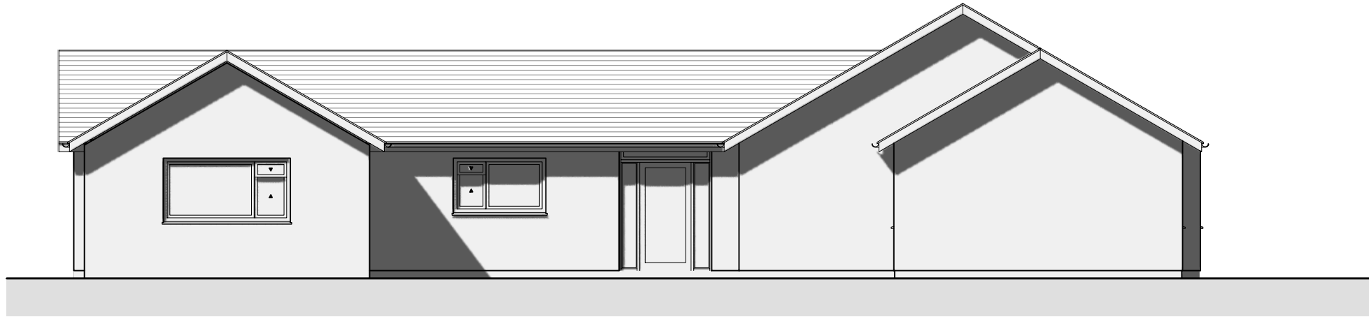
North Elevation
