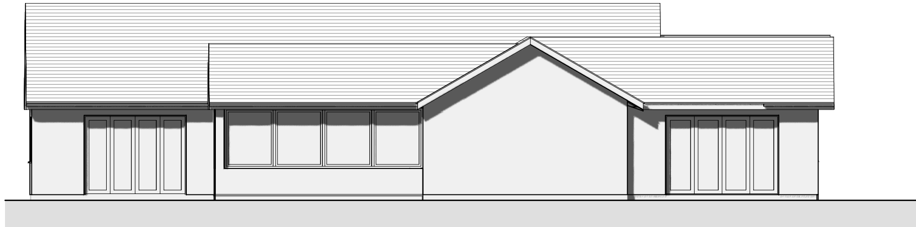
East Elevation
