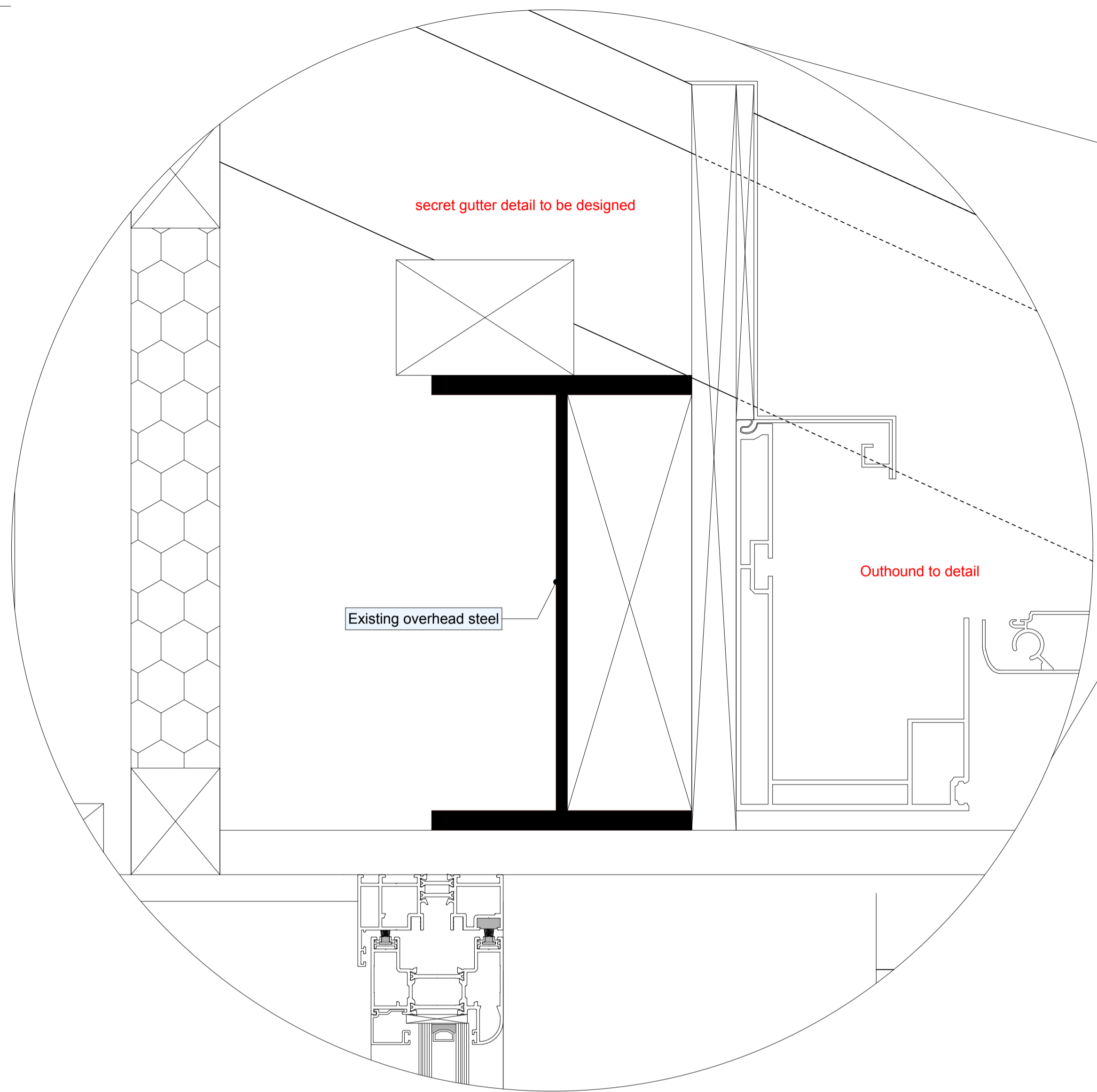
BALCONY DETAIL 3 1:2
