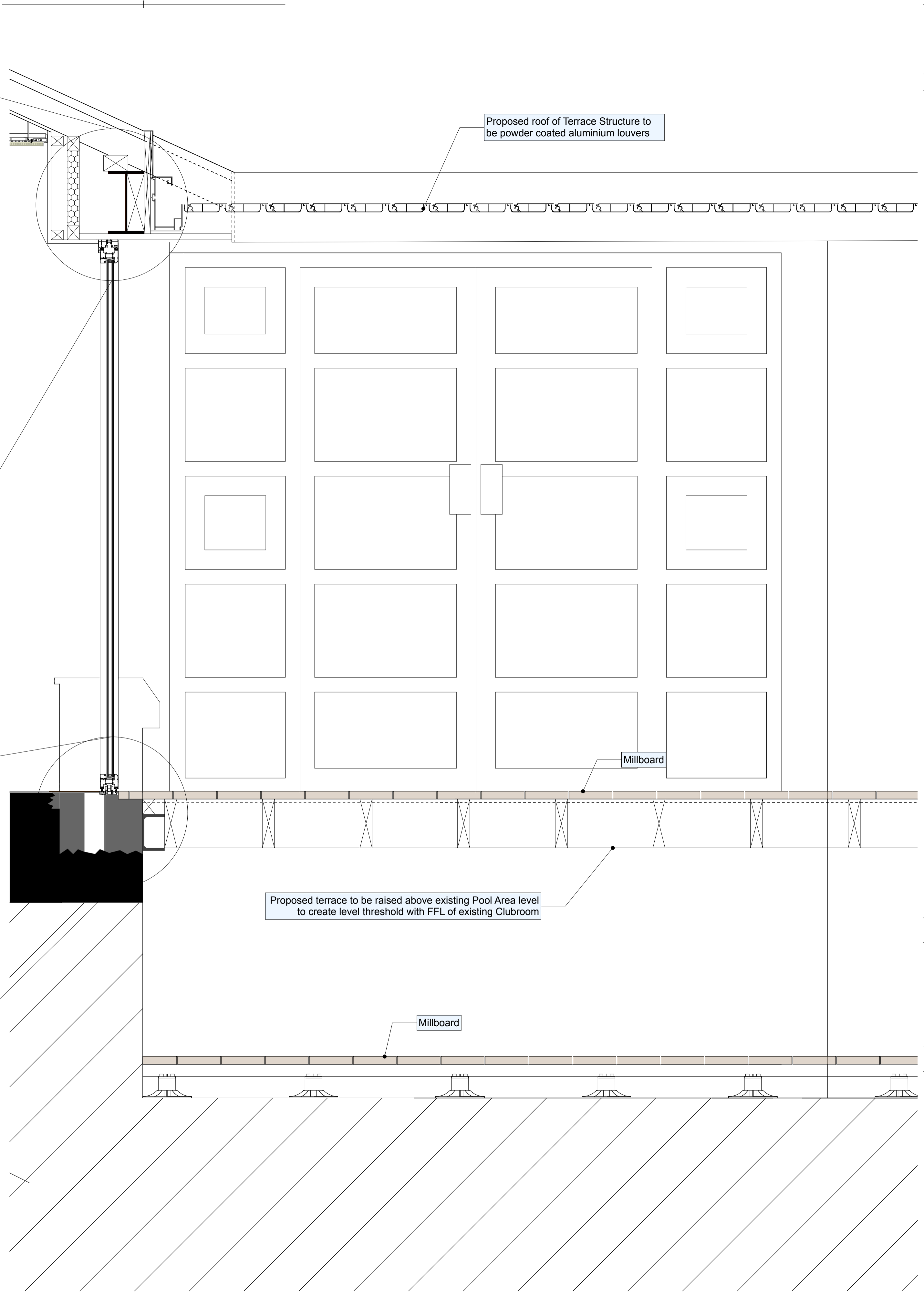
SECTION 1:10
