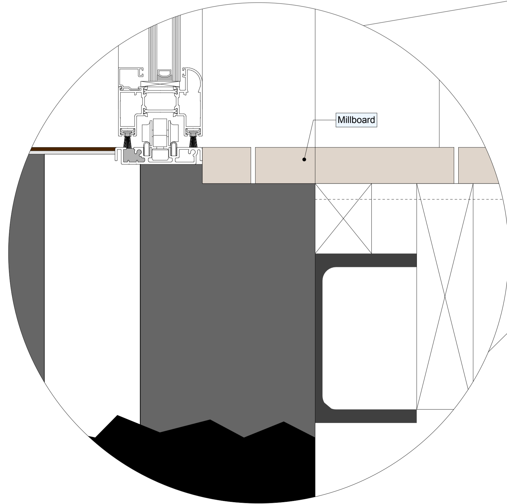
BALCONY DETAIL 4 1:2
