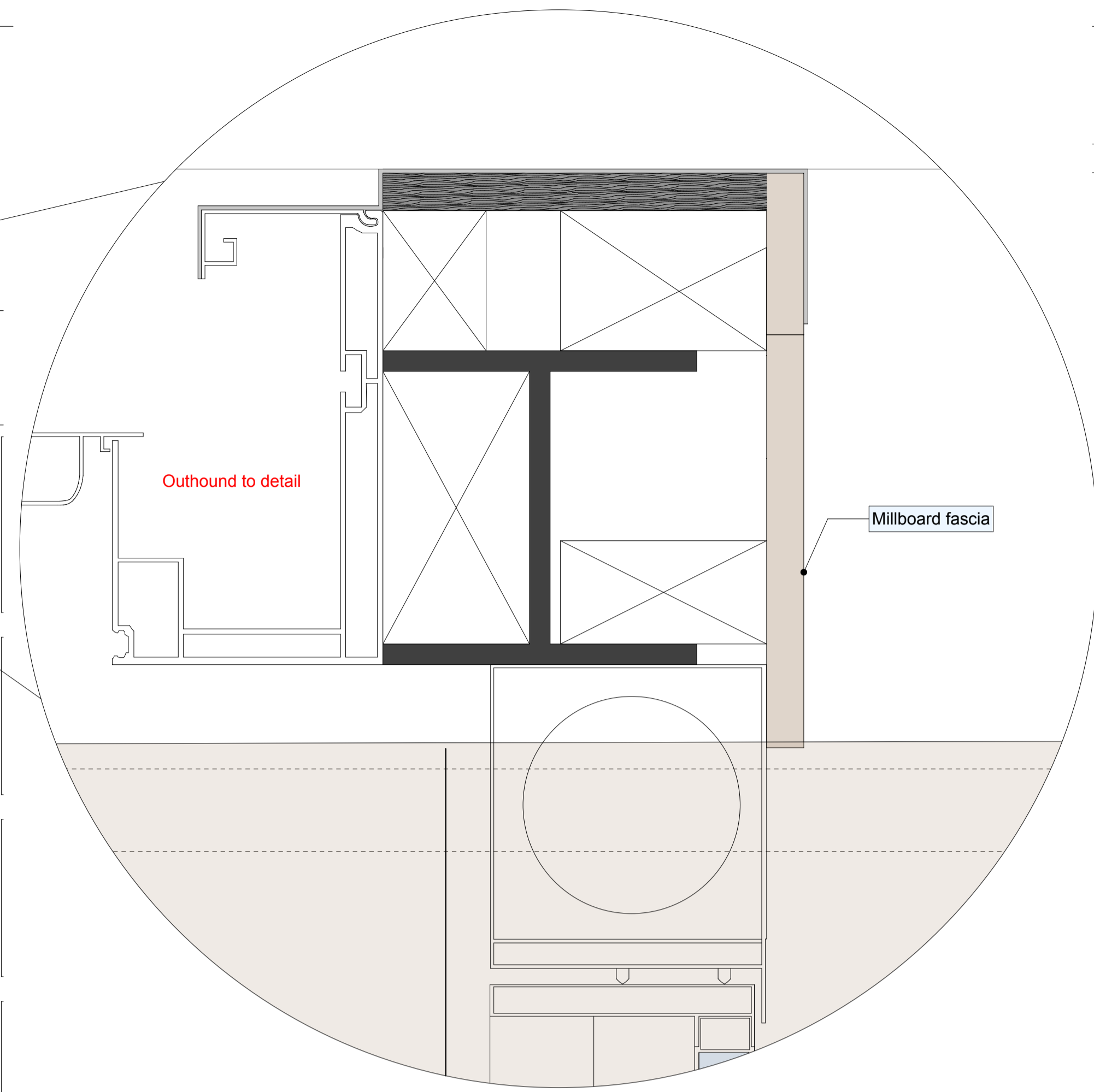
BALCONY DETAIL 5 1:2
