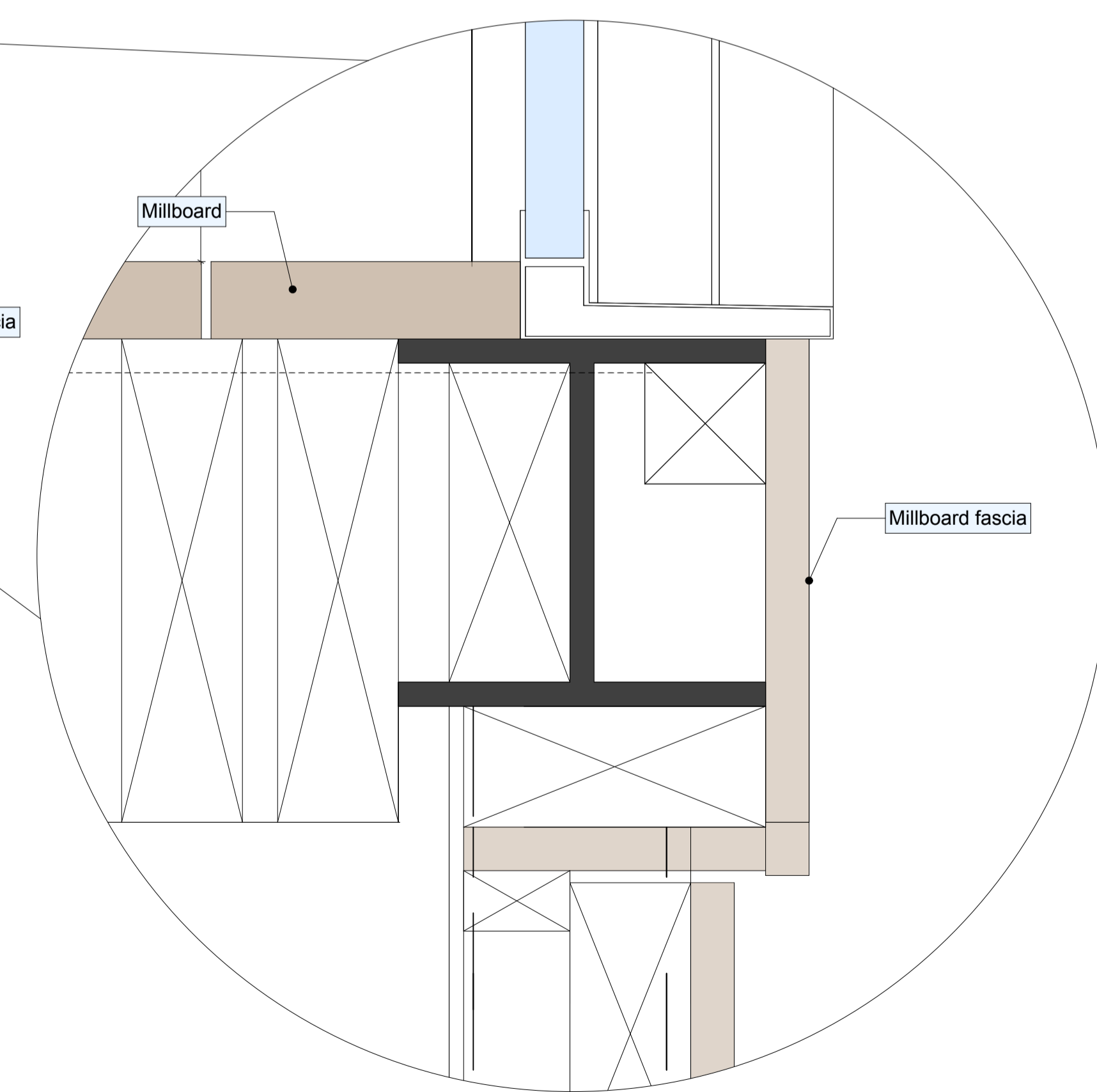
BALCONY DETAIL 6 1:2
