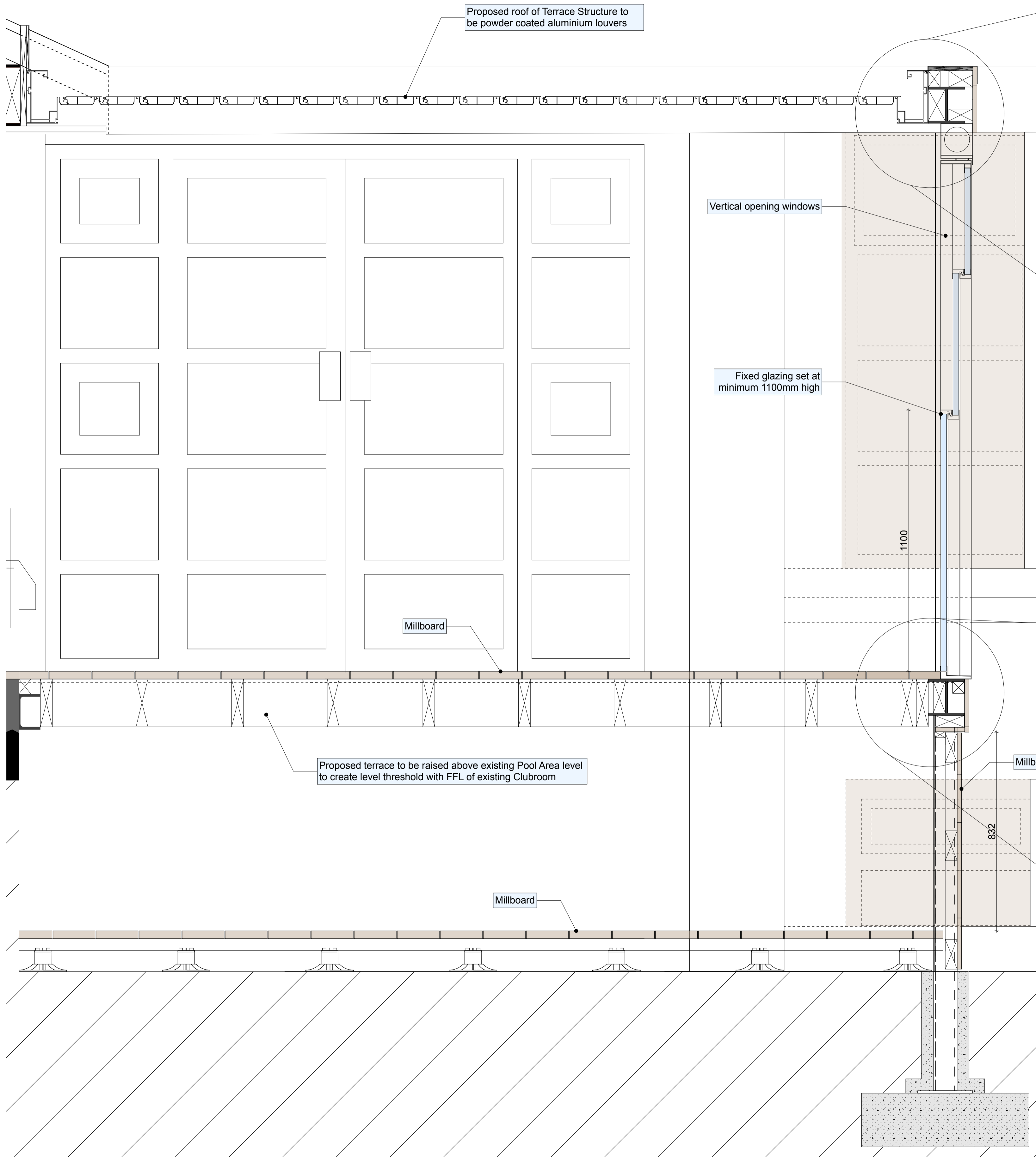
SECTION 1:10
