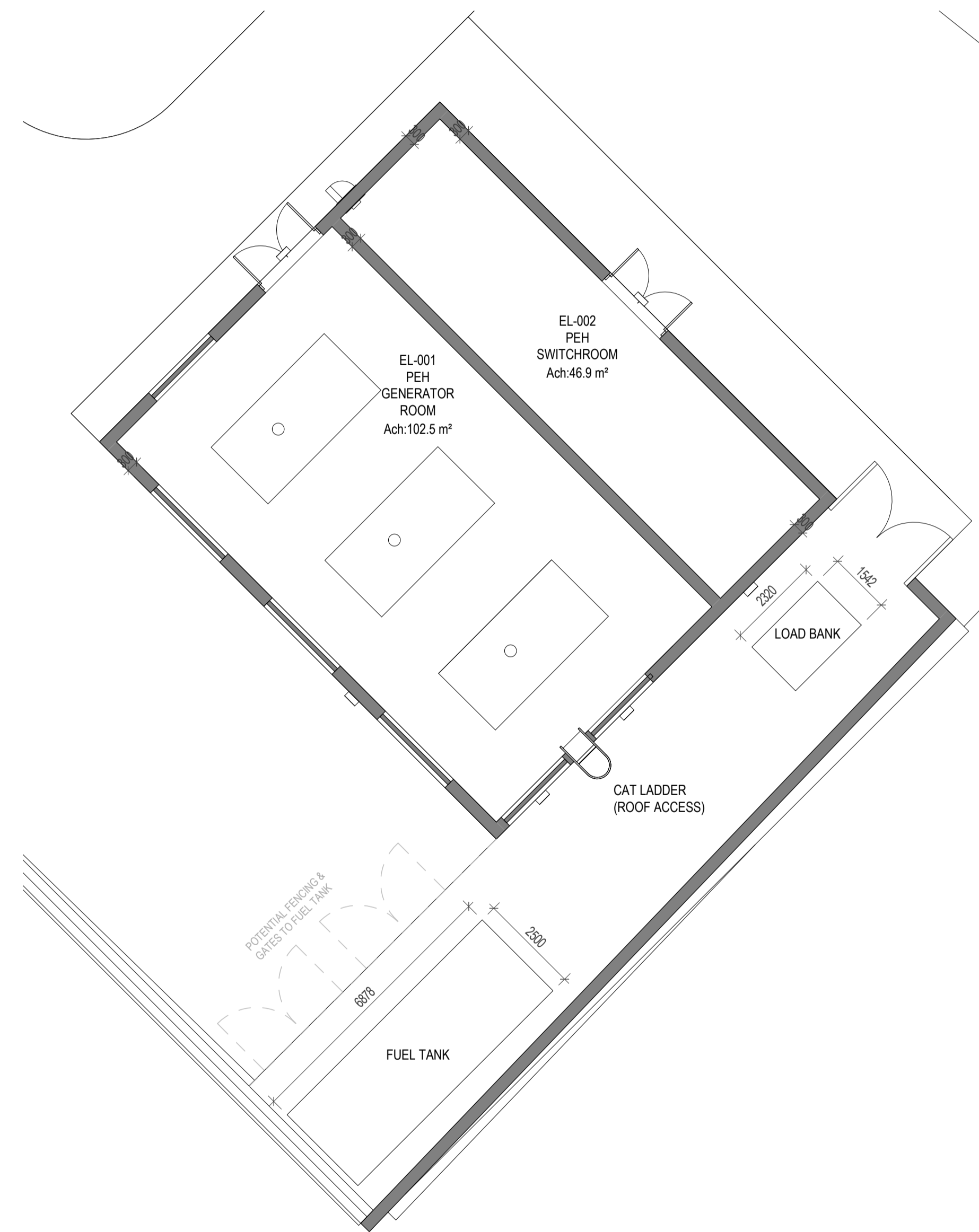
2 SUBSTATION BUILDING 2 (PEH) 1 : 100
