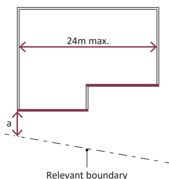
Diagram 13.7 Permitted unprotected areas in small residential buildings
