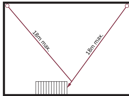
Basement or first storey
