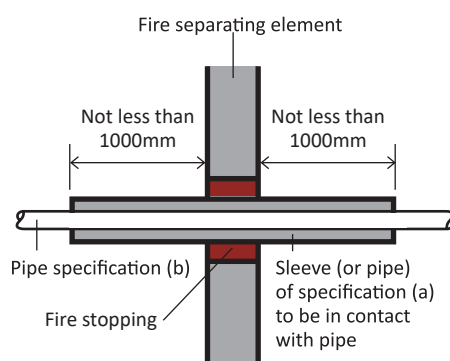
Diagram 10.1 Pipes penetrating structure
