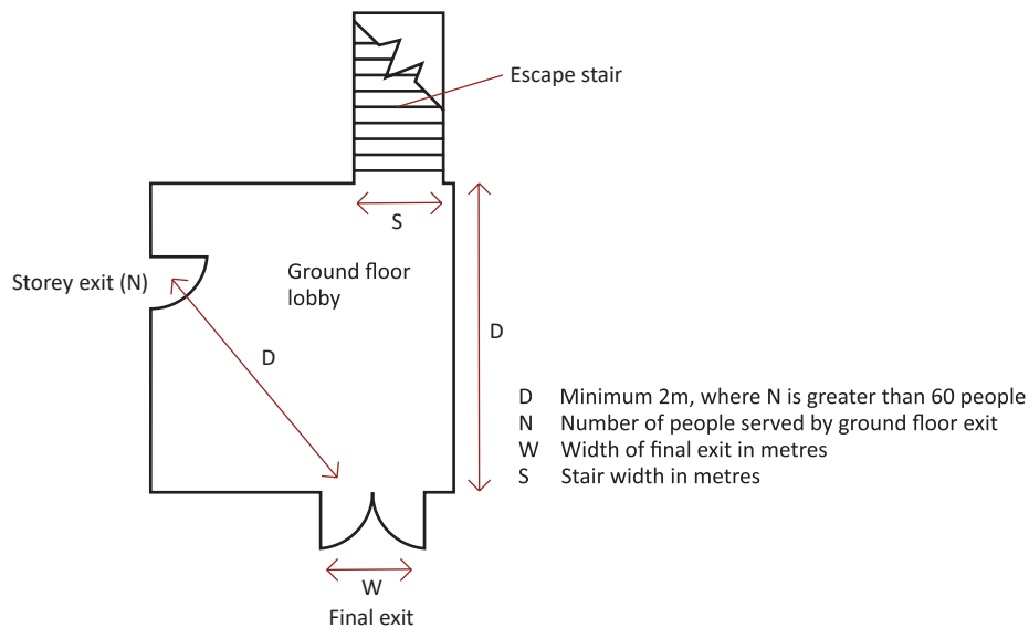
Diagram 2.6 Merging flows at final exit
