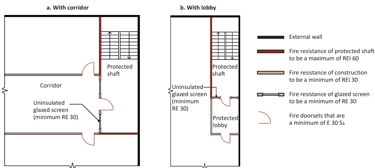
Diagram 8.4 Uninsulated glazed screen separating protected shaft from lobby or corridor
