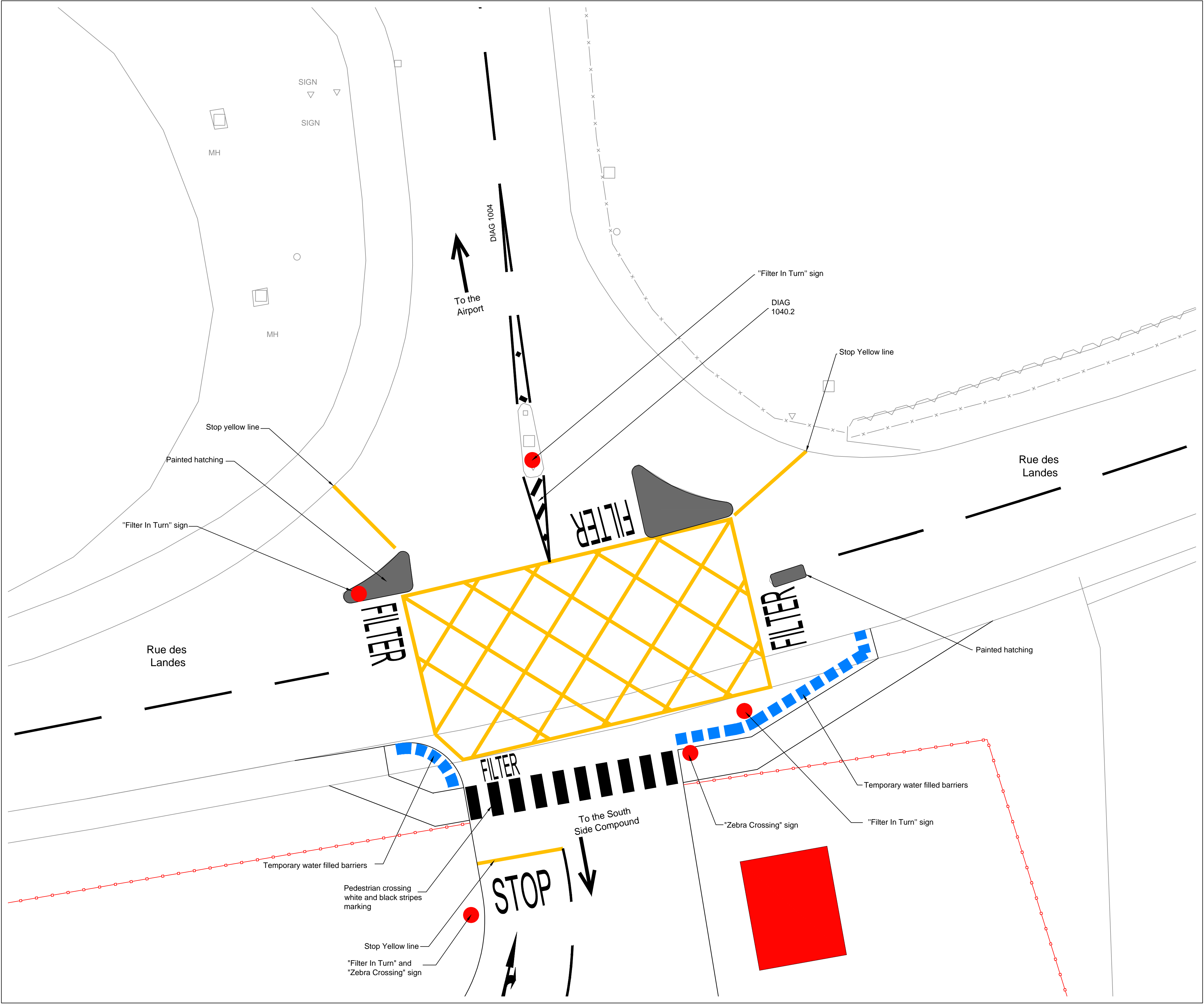
Junction Plan Scale: 1:100
